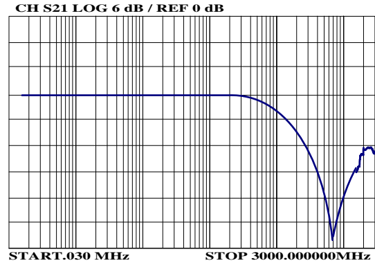
Figure 2: Insertion Loss
